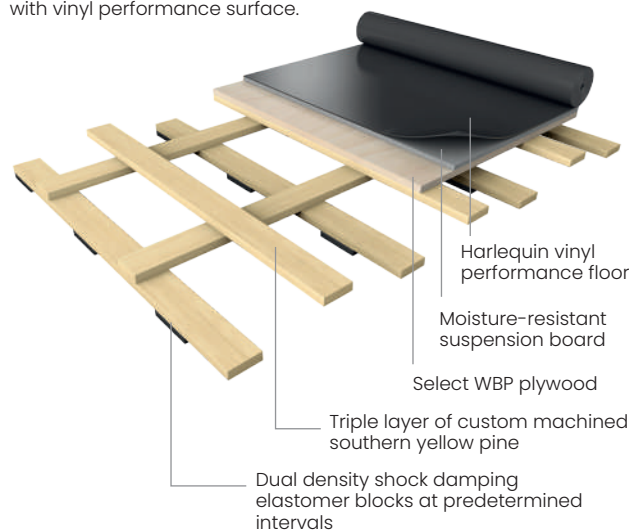
Harlequin WoodSpring sprung floor with vinyl performance surface.
